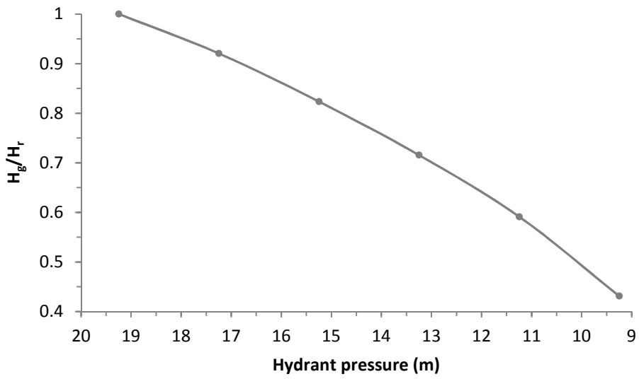
Figure 8. Relationship between \frac{H_g}{H_r} and hydrant pressure in scenarios B and C.
