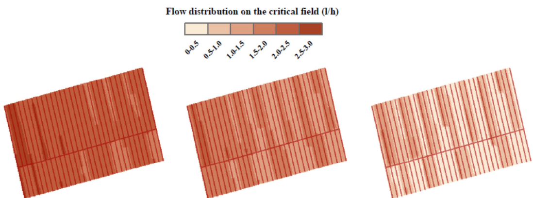
Figure 7. Spatial flow distribution of the non-compensating emitters in the critical field in the scenarios A and B for 33 (a), 27 (b) and 21 (c) m, respectively, of pressure at the pumping station.
