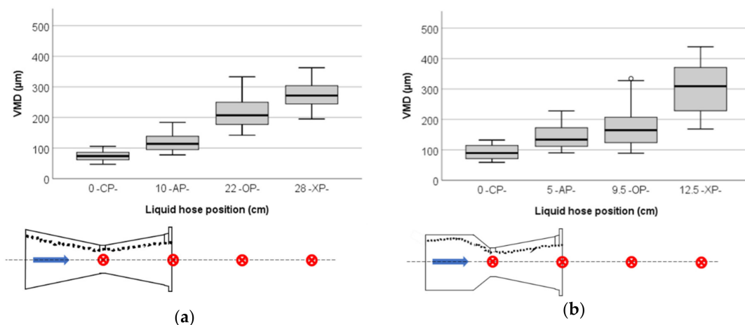
Figure 5. Volume Median Diameter (VMD) ( \mu\text{m} ) per liquid hose position (HP): (a) cannon-type and (b) hand-type spouts. CP, conventional insertion of liquid hose position; AP, alternative position; OP, out position; XP, extreme position.
