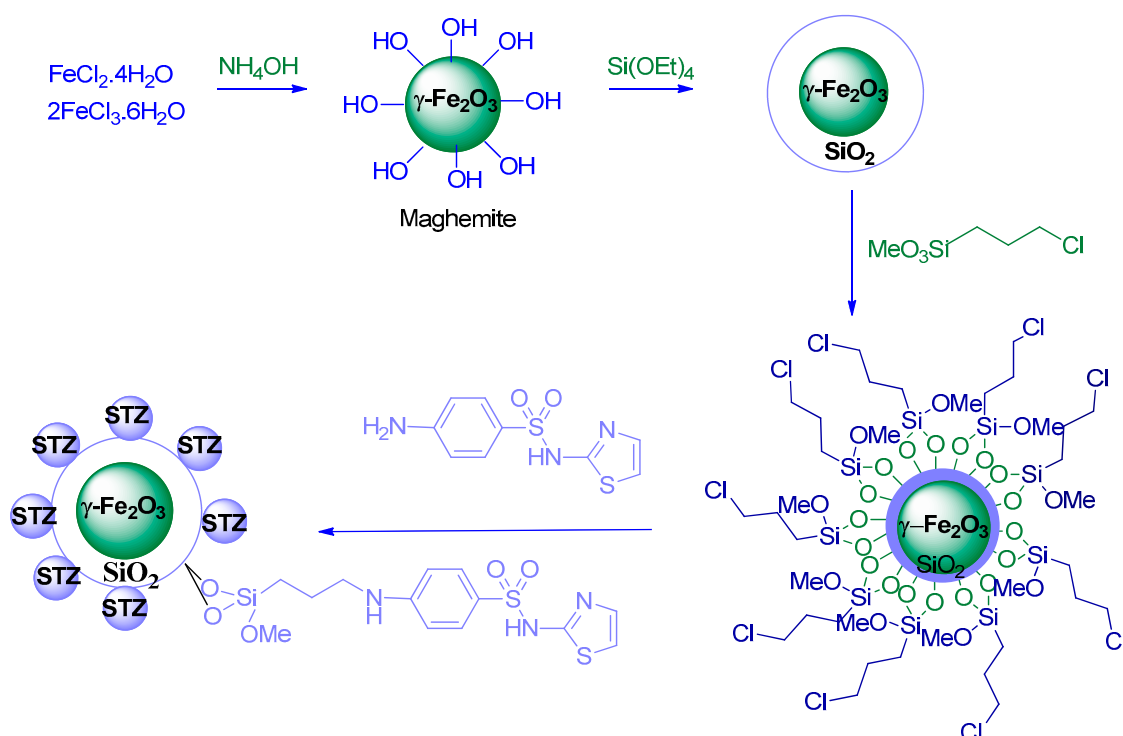
Scheme 2. Multistep strategy for the preparation of \gamma -Fe 2 O 3 /SiO 2 -STZ.
