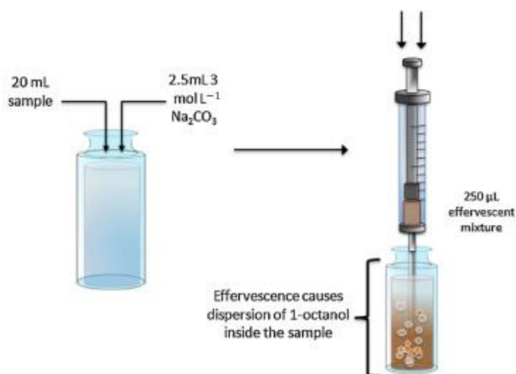
Figure 5. Schematic diagram of the effervescence-assisted dispersive liquid–liquid extraction (DLLME). Adapted with permission of Elsevier from reference [42].
