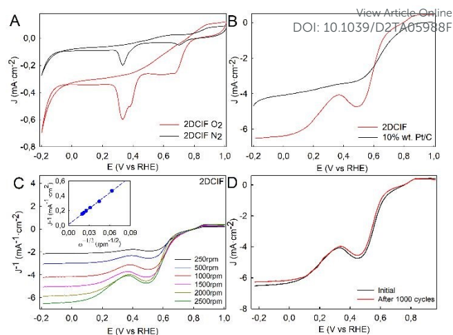
Fig. 3 (A) CV curves obtained for GCE modified with 2DCIFs in O 2 -saturated and N 2 -saturated 0.1 M KOH. (B) RDV curves of GCE/2DCIFs and GCE/10wt% Pt/C at the rotation rate of 2500 rpm in O 2 -saturated 0.1 M KOH. (C) RDV curves of GCE/2DCIFs at different rates (scan rate: 10\text{ mV}\cdot\text{s}^{-1} ). Inset: K-L plot ( J^{-1} vs \omega^{-1/2} ) for the 2DCIFs at 0.00 V. (D) CV curves of GCE modified of GCE/2DCIFs before and after 1000 cycles of the AAT, in O 2 -saturated 0.1 M KOH at scan rate of 10\text{ mV}\cdot\text{s}^{-1} and using a rotating rate of 2500 rpm.
