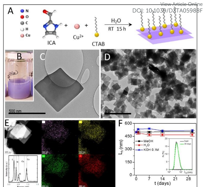
Fig. 1 (A) Synthetic scheme of 2DCIFs nanosheets. (B) Photograph of 2DCIFs dispersed in methanol. (C, D) TEM micrographs of the as-prepared nanosheets. (E) HAADF-STEM image and EDX elemental mapping displaying the uniform distribution of O (purple), Cu (green), N (yellow), and C (red) in the nanosheets (scale bar 200 nm). (F) Mean hydrodynamic lateral length L_h (mean value \pm SD) of 2DCIFs during 1 month immersed in different media (MeOH, Milli-Q water, and KOH 0.1M). The inset shows the DLS spectra of 2DCIFs in MeOH freshly prepared and after 1 month storage at 4 °C.
