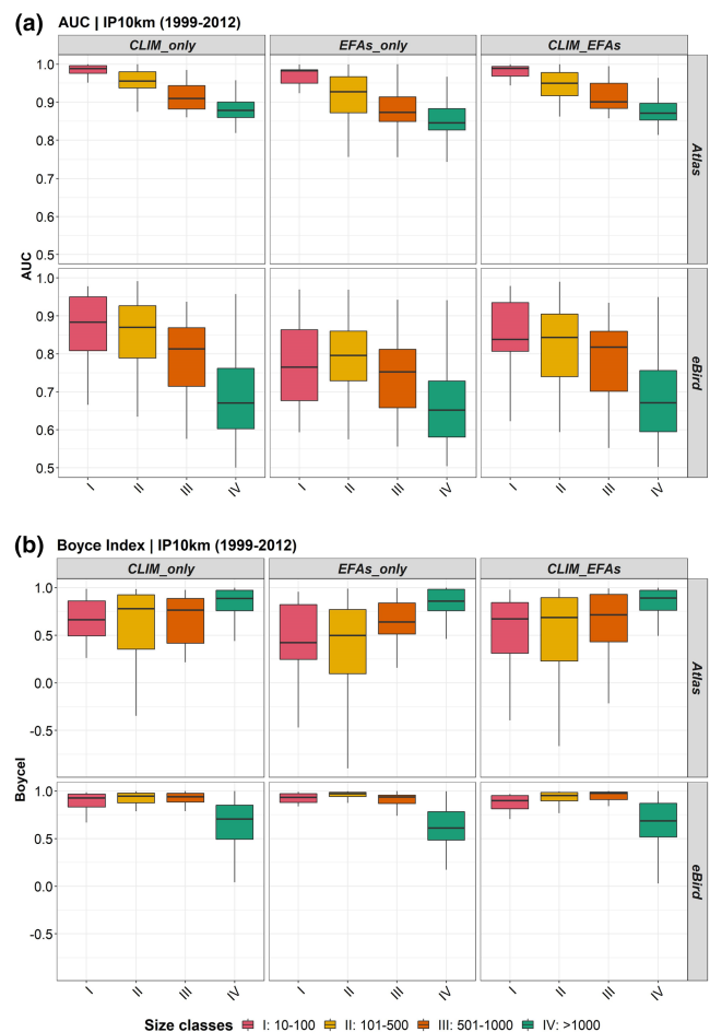
FIGURE 2 Comparison of relative performance of the (a) area under the curve (AUC) and (b) the Boyce's index (Boycel) between bird data source (Atlas vs. eBird) for the Iberian Peninsula, type of predictor (CLIM_only, EFAs_only and CLIM_EFAs) and size class (I: 10–100; II: 101–500; III: 501–1000; IV: >1000) for the top-ranked ensemble models. The boxplots represent the performance of individual models per size class showing the AUC_{\text{median}} and Boycel_{\text{median}} , two hinges (first and third quartiles), and two whiskers of each model. Number of species per dataset = 236
