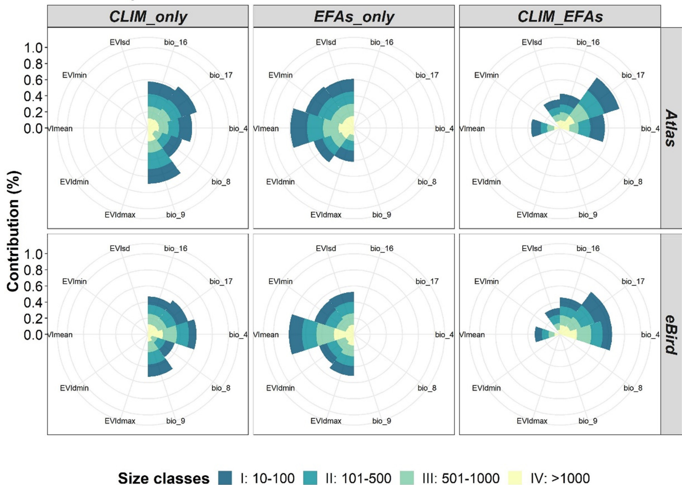
FIGURE 3 Relative variable contribution (%) across all models for the three groups of predictors, CLIM_only (precipitation and temperature), EFAs_only (primary productivity, seasonality and phenology) and the combined group (CLIM_EFAs), per each bird data source and size class for the Iberian Peninsula. See Table S1 in Appendix S1 to check the codes and description of each predictor. EFA, ecosystem functional attribute
