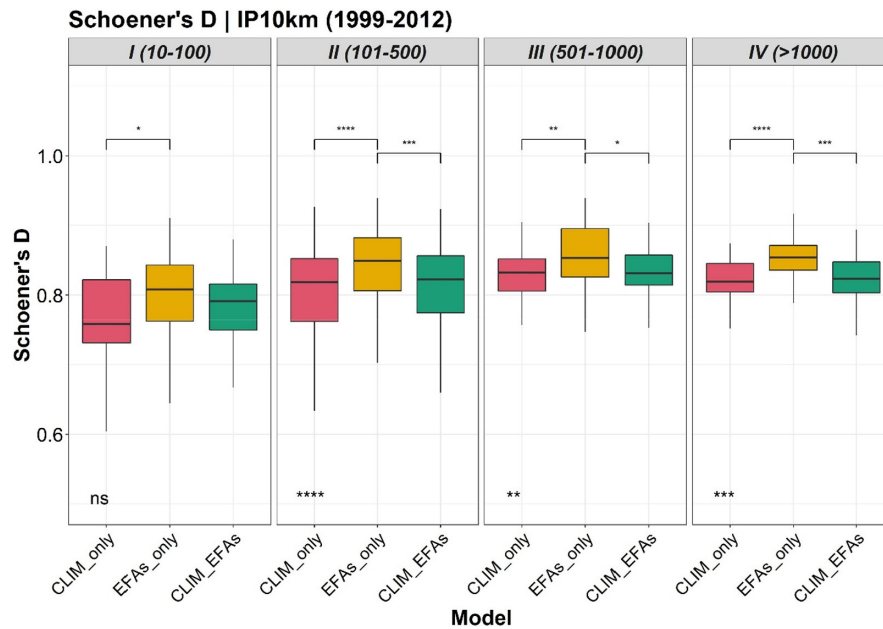
FIGURE 4 Similarity test between size classes based on pairwise species niche overlaps from both Atlas and eBird datasets, and from the spatial projections of the three sets of models (CLIM_only, EFAs_only and CLIM_EFAs) for the Iberian Peninsula. For all box plots, the lower and upper whiskers encompass the 95% interval, the lower and upper hinges indicate the first and third quartiles, and the central black line indicates the median value of the Schoener's D index. The D value ranges from 0 (no overlap) to 1 (identical predictions). The symbols (*), (**), (***) and (****) indicate significant differences based on the Kruskal–Wallis test at the bottom of boxplots, and the one concerning pairwise comparison on top of boxplots ( p = 0.05 , p = 0.01 , p = 0.001 and p = 0.0001 , respectively). EFA, ecosystem functional attribute
