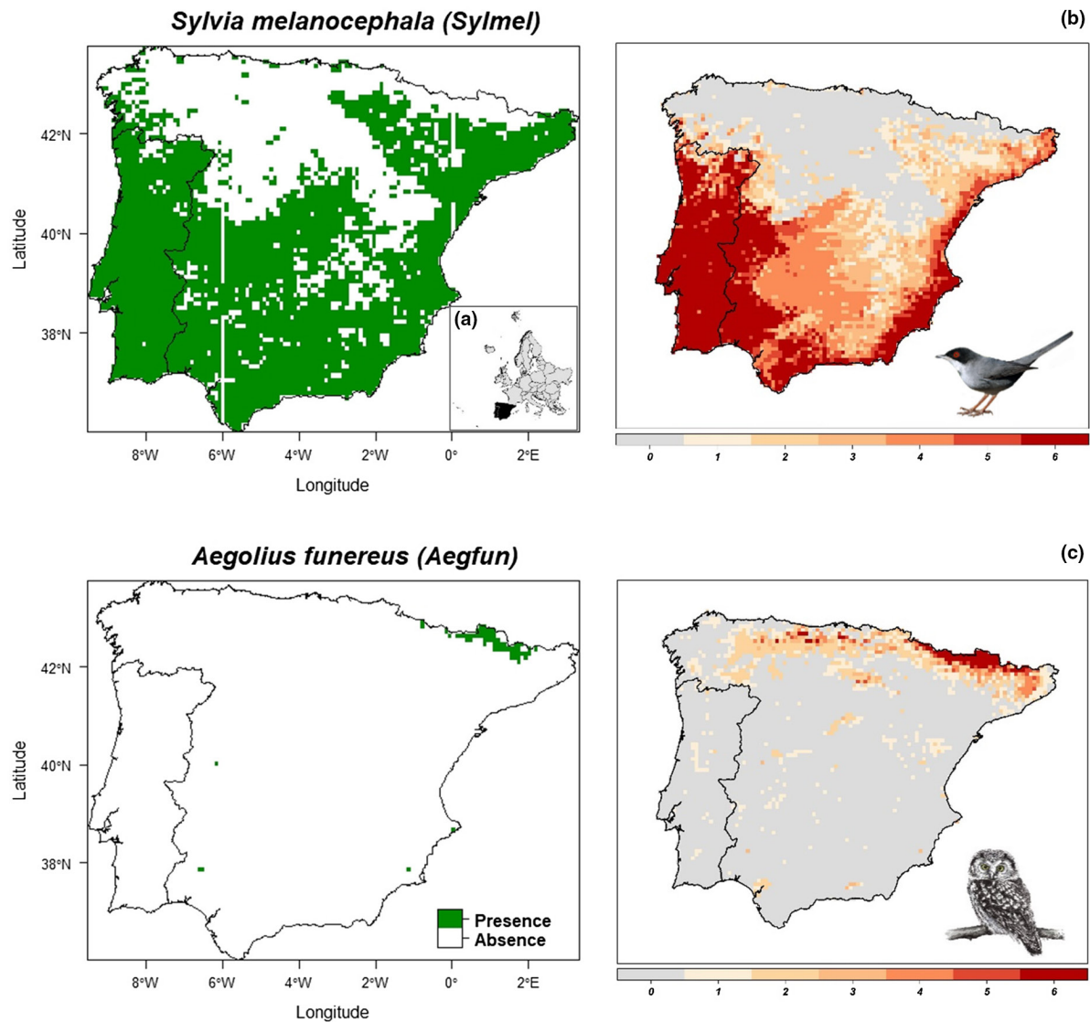
FIGURE 5 Examples of species presences/absences in the Iberian Peninsula in Europe (a), and degree of overlap among maps from the Atlas and eBird datasets and the three group of predictors (CLIM_only, EFAs_only and CLIM_EFAs) for (b) a widely (Sardinian warbler, Sylvia melanocephala ) and (c) a narrowly (boreal owl, Aegolius funereus ) distributed species. The colour ramp of compatibility maps ranges from grey = 0 (no models) to dark red = 6 (all models). See maps for all species in Figure S3.4 in Appendix S3. Geographical coordinate system of this map is WGS 84. EFA, ecosystem functional attribute
