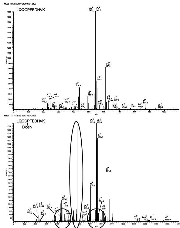
Figure 1: Fragmentation spectra of a non biotinilated (upper panel) and a biotinilated peptide (lower panel) showing the presence of multiple fragments produced by biotin that could not be assigned (circles).
