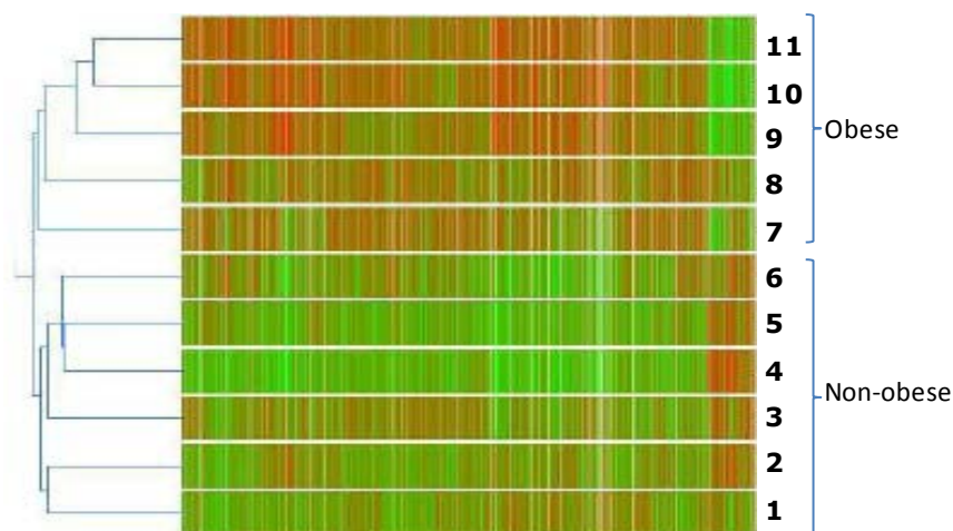
Figure 2. Microarray analysis of the transcripts expressed in the visceral adipose tissue from obese vs. normal-weight (control) prepubertal children. RNA from each patient was subjected to chip analysis using Affymetrix Human Genome U133Plus 2.0 GeneChips. The normal-weight group consists of six individuals (numbers 1–6), and the obese group consists of five patients (numbers 7–11). Bidimensional cluster analysis was performed using a Pearson correlation. The parametric test ANOVA was used to uncover the 1588 genes that were differentially expressed.
