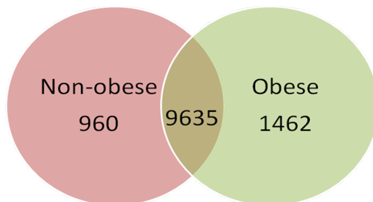
Figure 1. Venn diagram of the expressed sequences in the visceral adipose tissue of obese and normal-weight prepubertal children. After filtering the data with the Affymetrix Detection Algorithm, a total of 12,057 sequences were found to be expressed in adipose tissue. Each condition is represented by a circle in the Venn diagram. The numbers in the region of the overlapping circles indicate the genes that are expressed in both conditions.
