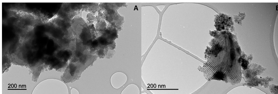
Figure 3. TEM images of (A) 40% FeMagC at 400 °C, and (B) 40% FeMagN at 400 °C.
