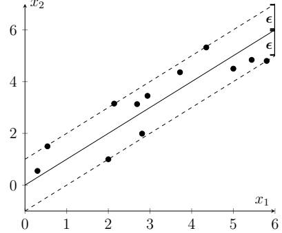
Fig. 2.4.: Linear support vector regression example solution on a toy 2D dataset.
