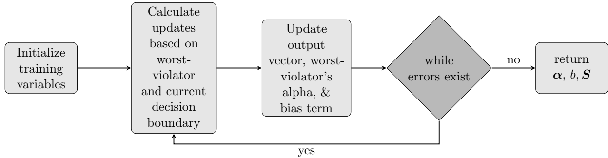
Fig. 5.1.: A summary of the steps performed by OLLAWV. The model parameters (\alpha, b, \mathcal{S}) and the algorithm variables (\mathbf{o}, t, wv, \text{ and } y_o) are first initialized. The worst-violator with respect to the current hyperplane is then found and the model parameters are then updated. Once no more violating samples are found, the model is returned.
