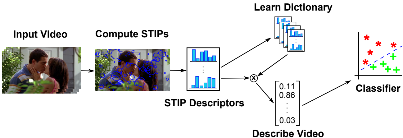
Fig. 4: Classical pipeline for learning with BOW : (i) Compute STIP on input video; (ii) compute descriptors from STIP; (iii) learn a dictionary of visual words; (iv) describe video by using STIP descriptors and learnt dictionary; and, (v) train a discriminative classifier.
