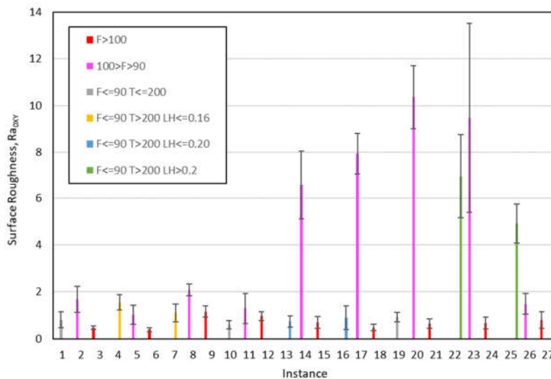
Figure 11. Mean values and standard deviation for R_{a,0,XY} ; each color represents a leaf of the decision tree: pink, yellow and green instances belong to class 2; the rest of color belong to class 1 (F: Flow; T: Temperature; LH: layer height).
