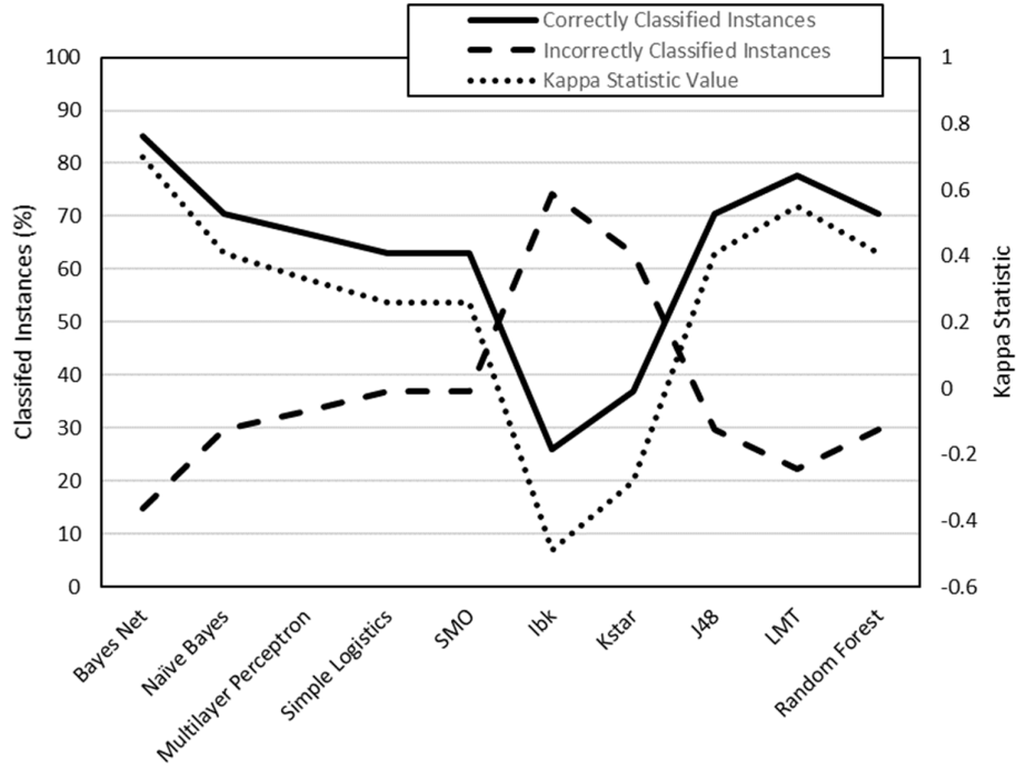
Figure 4. Evaluation of the models generated by WEKA for R_{a,90,XY} data (cross-validation, 10 folds).
