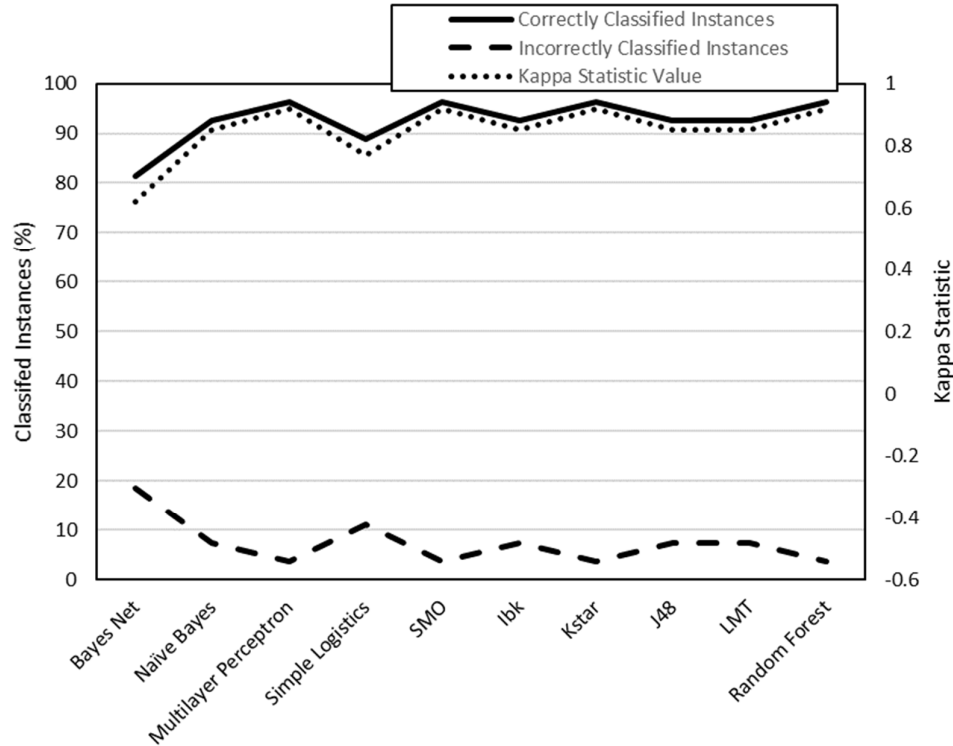
Figure 6. Evaluation of the models generated by WEKA for R_{a,9,0xz} data (cross-validation, 10 folds).
