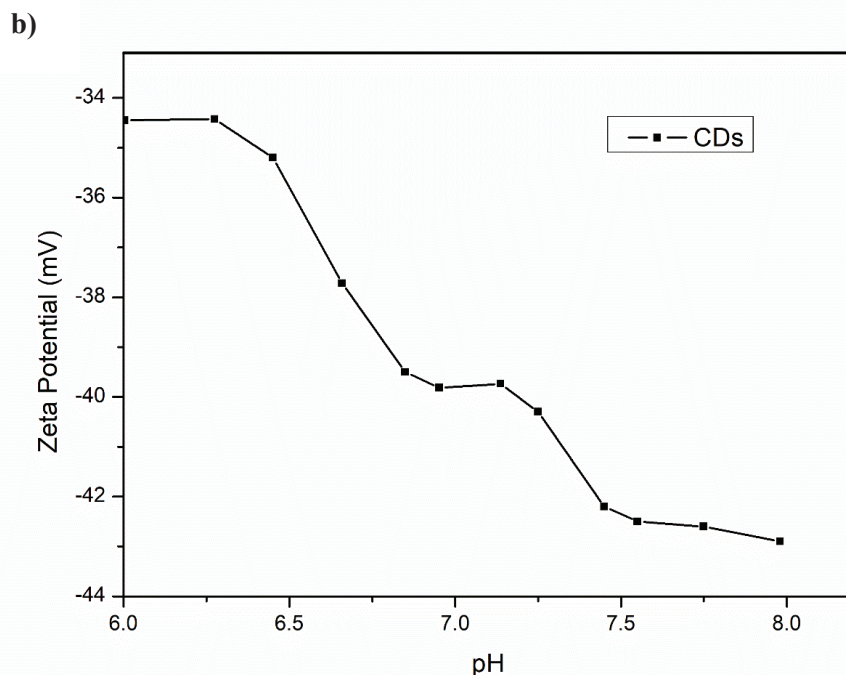
Figure 3.1.4. a) DLS size distribution and b) zeta potential at different pH values of CDs
