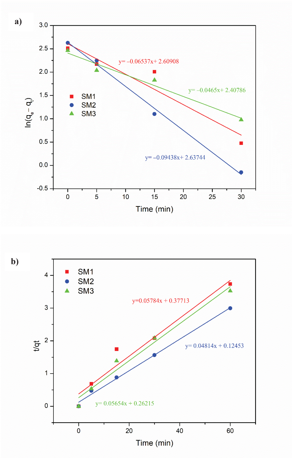
Figure 3.5.12. Kinetic of Rhodamine B adsorption by SM1, SM2, and SM3, fitted by a) pseudo-first order model and b) pseudo-second order model.
