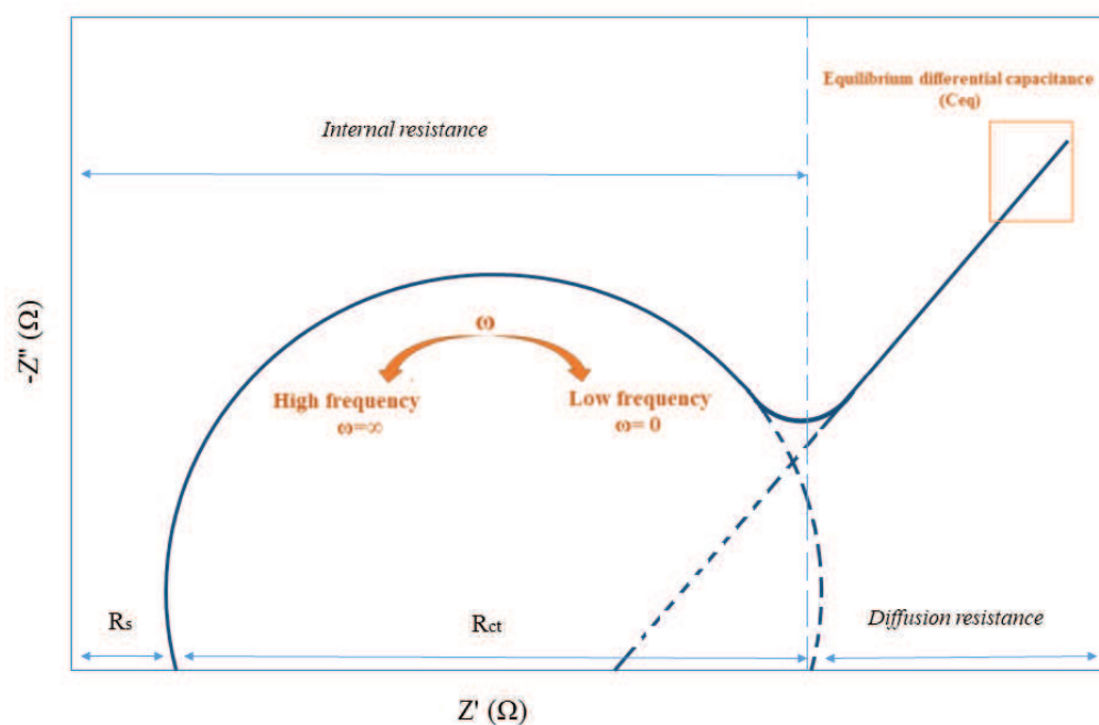
Figure 2.16. Nyquist diagram
