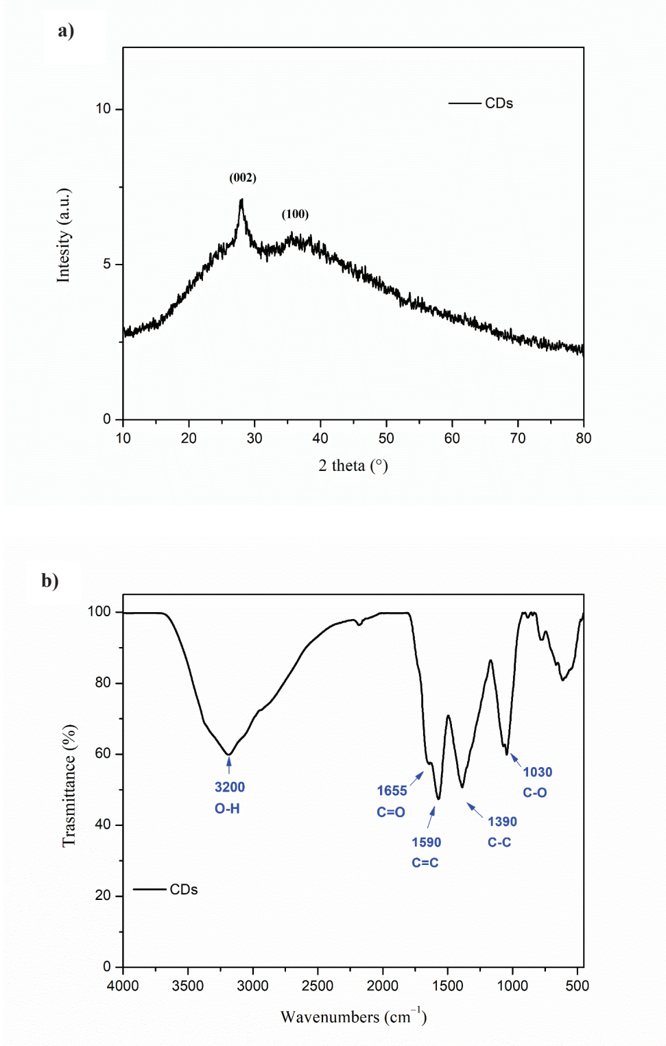
Figure 3.1.5. Compositional analysis of CDs: a) XRD spectrum; b) FTIR spectrum
