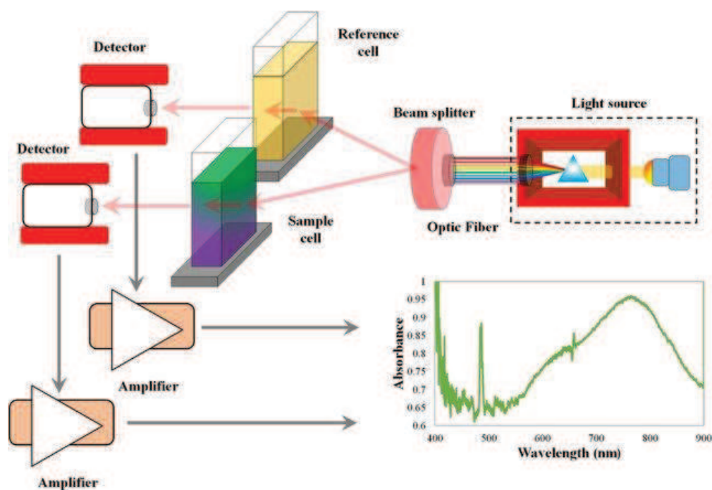
Figure 2.13. Schematic of UV-Vis setup (Ashraf Gandomi et al. , 2018)
