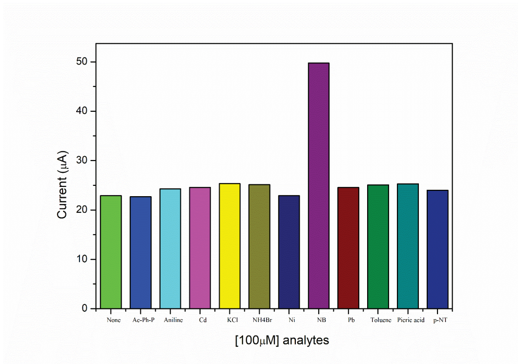
Figure 3.1.15. Histogram response of the CDs/SPCE at the addition of organic and inorganic interferences in solution (0.01M PBS at pH 7.4) at a concentration of 100 \mu M each (scan rate of 200mV/s)
