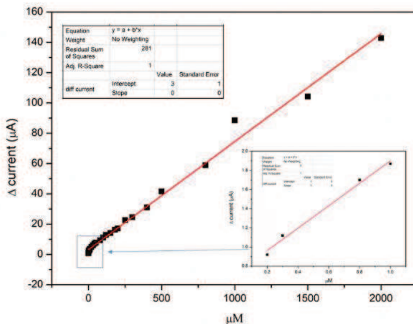
Figure 3.1.14. a) DPV of CDs/SPCE in 0.01 M PBS electrolyte and at different concentrations (0.1–2000 \mu\text{M} ) of NB; b) calibration graphs for peak reduction currents, \text{sd} \leq 2 .
