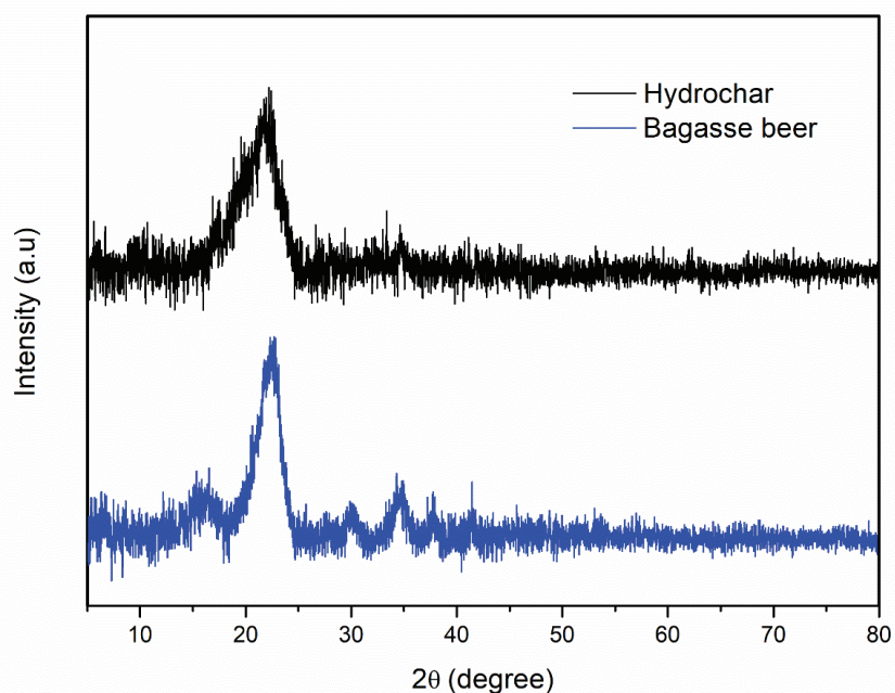
Figure 3.2.3. XRD spectra of bagasse beer (blue) and hydrochar (black) after background removal
