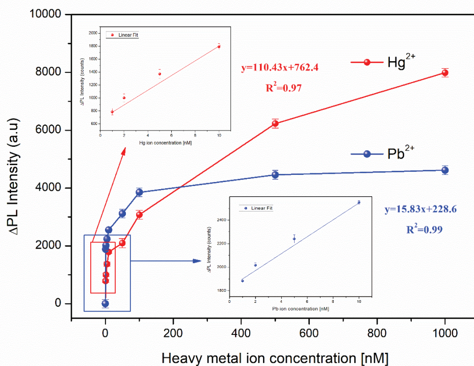
Figure 3.2.15. CNDs PL response to Hg 2+ and Pb 2+ addition in nanomolar concentrations range
