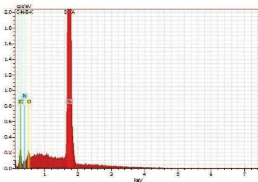
Figure 3.1.3. EDX spectrum
