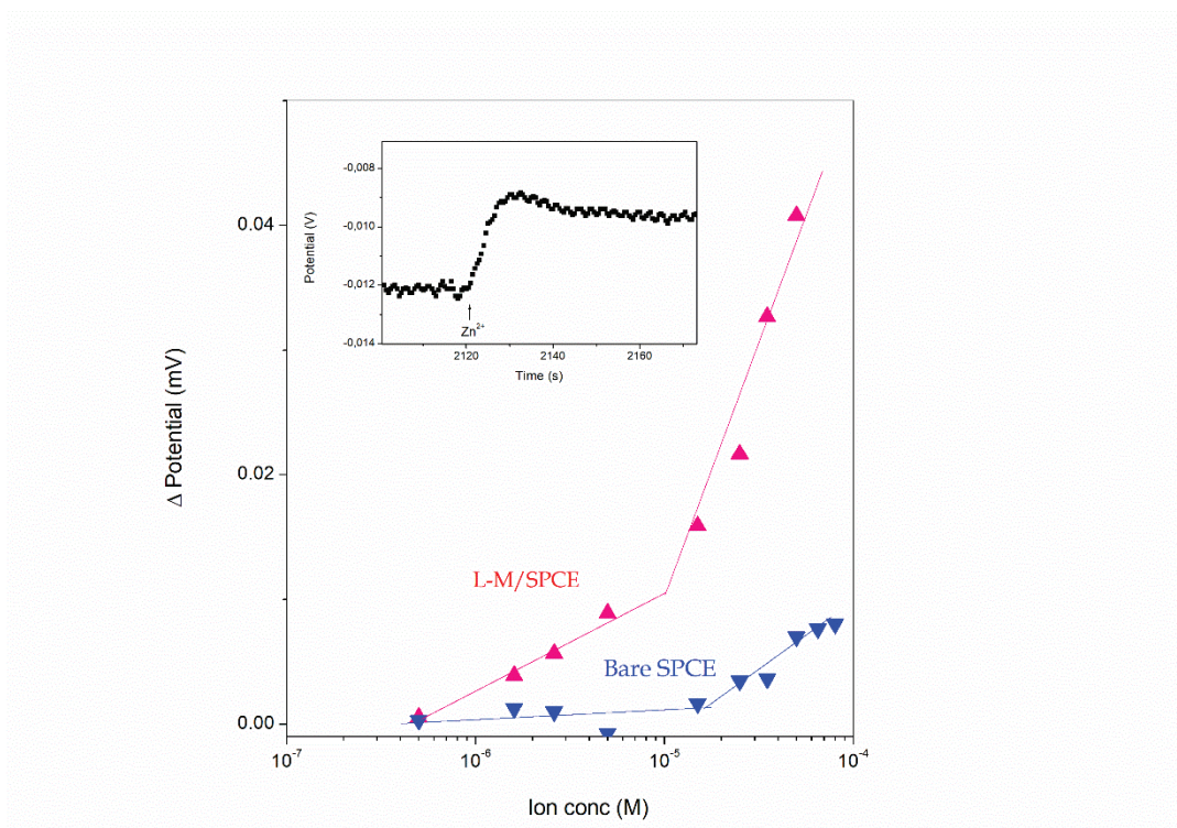
Figure 3.4.10. Calibration curves for the bare SPCE and L2-M/SPCE sensor to different concentrations of Zn ions. Dynamic response time of the L2-M/SPCE sensor for a step change in the concentration of Zn 2+ ion
