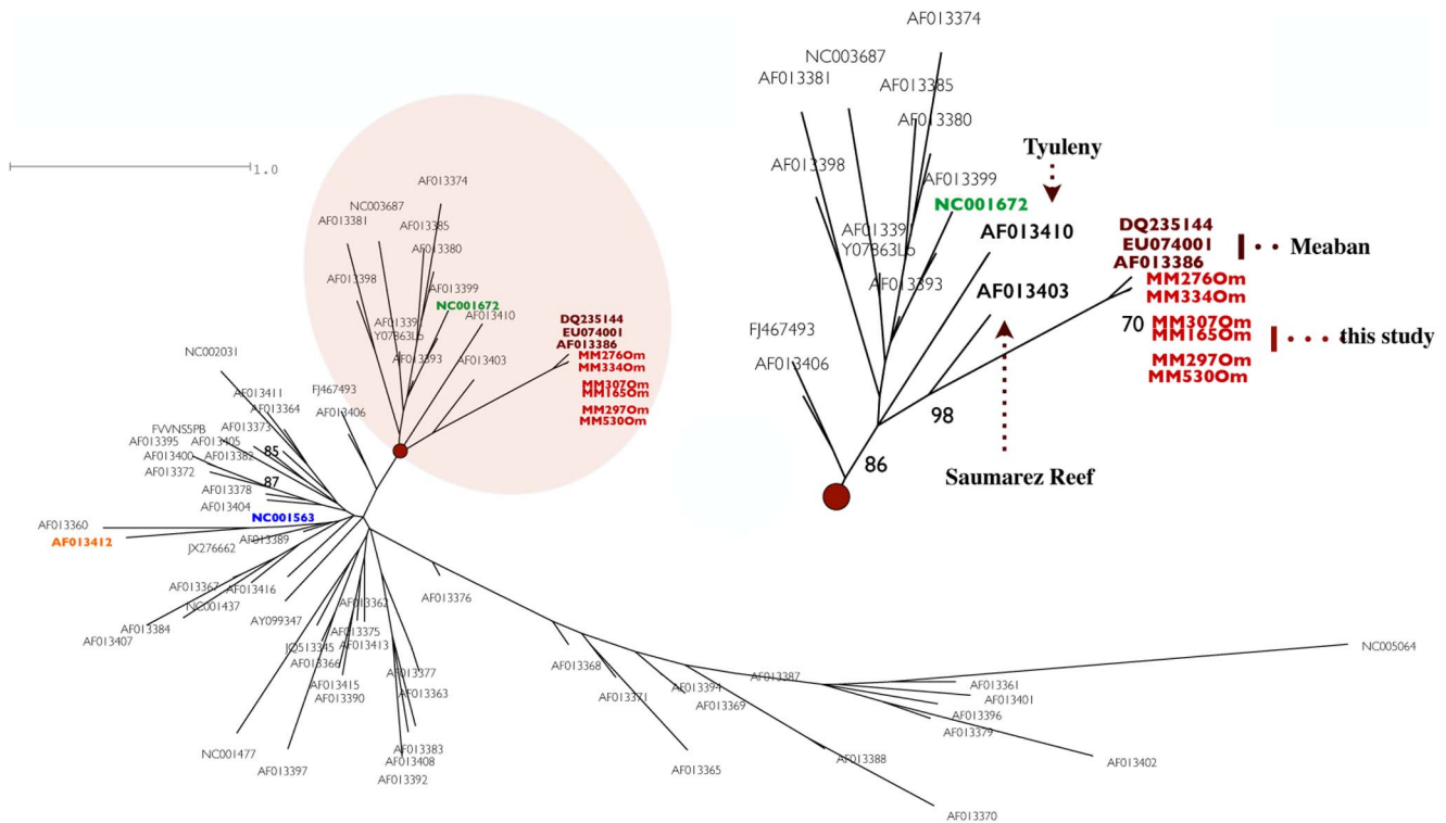
Figure 2. Unrooted maximum-likelihood tree constructed using NS5 partial gene sequences (143 bp) amplified from O. maritimus ticks (red) and a set of sequences from the flavivirus complex (see text). Only bootstrap support values above 70% are indicated above the branches. Reference sequences obtained for viruses belonging to the seabird tick-borne flavivirus group are indicated; these include Meaban (red: this study, dark-red: reference), West Nile (blue), Usutu (orange), and tick-borne encephalitis (green). doi:10.1371/journal.pone.0089601.g002
