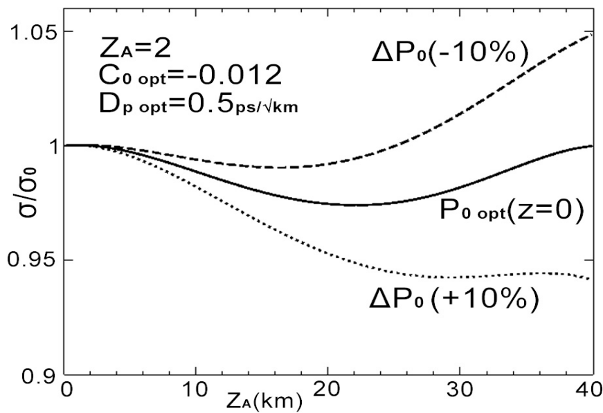
Figure 7. Evolution of the normalized widening with z_A = 2 in an amplification stage with different initial power peaks: optimal power (—), 10% over (···) and 10% under (---), in all the three cases shared between components according to (55) and (56) with \theta = \pi/4 and optimal chirp. The value for the PMD parameter is D_p = 0.5 \text{ ps} \cdot \text{km}^{-1/2} .
