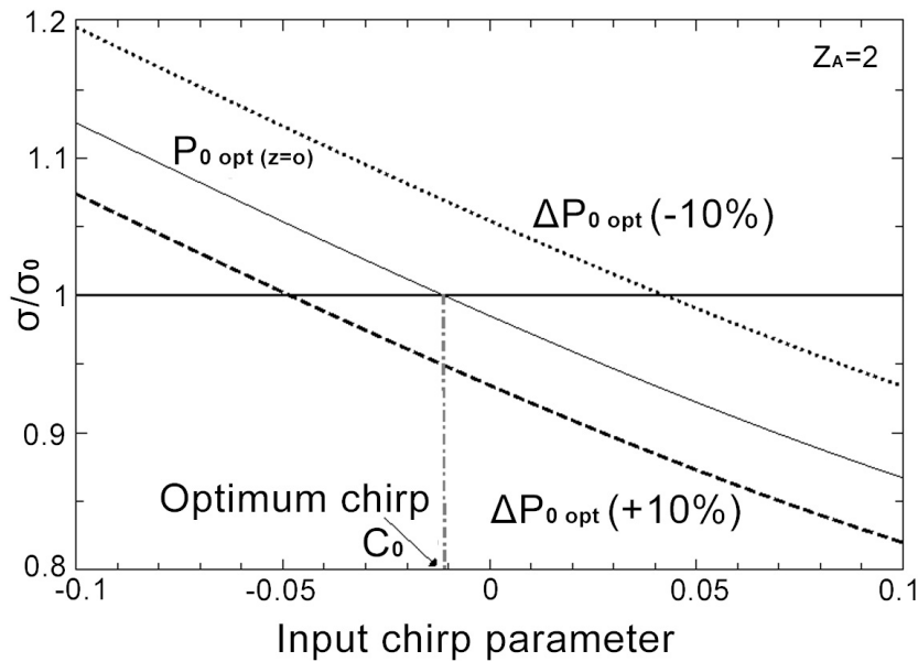
Figure 6. Change in the widening factor through an amplification stage for the vectorial soliton with z_A = 2.0 vs. the initial chirp, for different peak powers in z = 0 . We assume a PMD value of D_p = 0.5 \text{ ps} \cdot \text{km}^{-1/2} .
