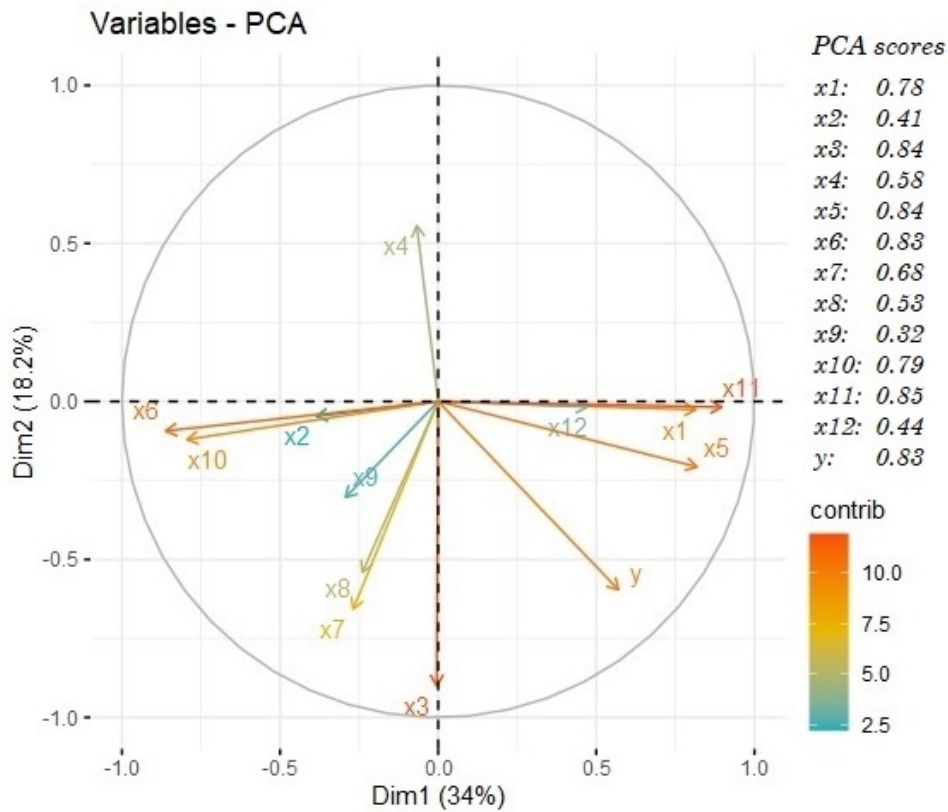
Figure A3. The principal component analysis (PCA) plot. Vectors are colored according to the contribution degree to LIF. PCA scores are equal to the module of each vector, indicating the weight associated with the combination of the two principal components (i.e., Dim 1 and Dim2, respectively explaining 34 and 18.2% of LIF variance). Variables are defined in Table 4.4.
