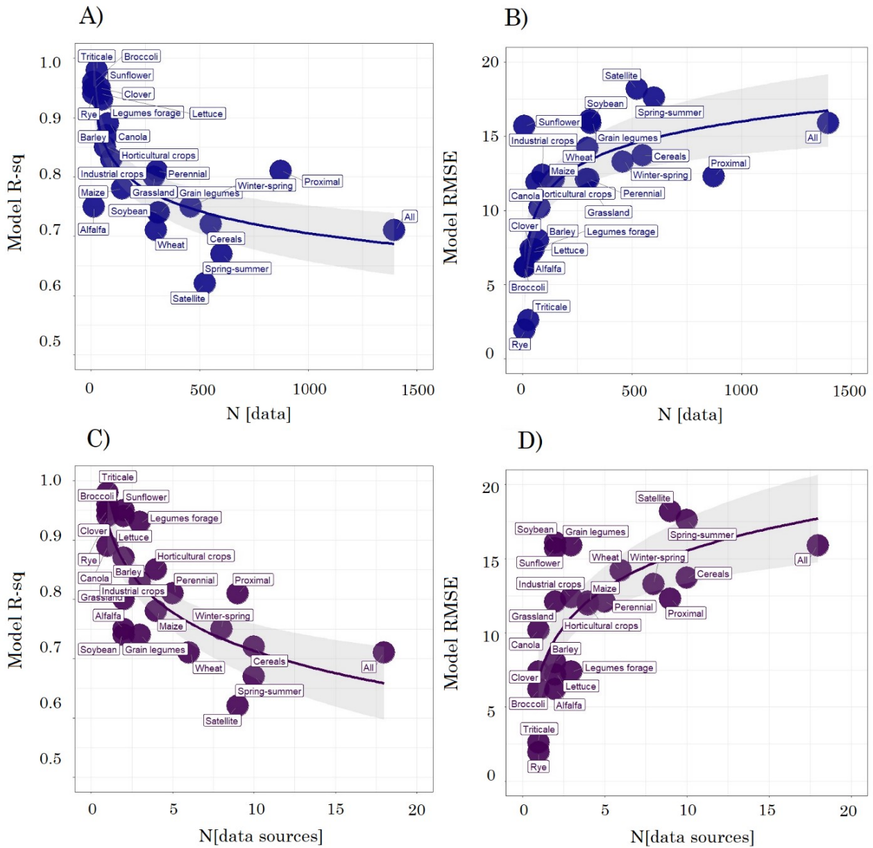
Figure 3.5: Statistical indicators of model performance: R^2 and RMSE plotted against sampling size (A and B, respectively) and against the number of data sources used for each model (C and D, respectively). Both indicators followed a logarithmic response curve, negative for the case of R^2 and positive for RMSE. All regression coefficients were significant and R^2 values ranged around 0.6 (results not shown).
