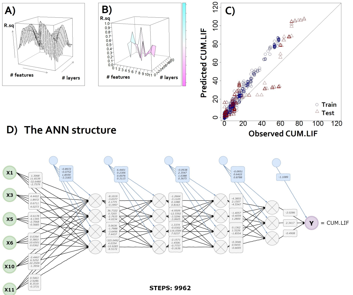
Figure 4.7: The feedforward Artificial Neural Network (ANN) used for forecasting lateral inflow (LIF) over 30 years: A) schematic representation of the R^2 assessment based on trial-and-error procedure that was taken for model architecture delineation; B) three-dimensional representation of the R^2 values obtained for each combination of model structure (the best performing ANN corresponded to an ANN composed by six different features and four hidden layers); C) ANN statistical evaluation, observed LIF plotted against predicted LIF (values are expressed in mm and represent cumulative LIF), blue dots correspond to the training set (2019/20) and red triangles to the testing set (2020/21). Both the training and the testing set fitted into a linear regression, respectively expressed as y = 1.432x + 0.528 and y = 1.122x + 2.919 , and subsequently with a R^2 of 0.97 and 0.78, and a RMSE of 10.1 and 14.8 mm; D) the schematic representation of the best performing ANN, solved in 9962 steps: green circles represent input features, grey squares indicate the hidden layers' coefficients, each node is represented by a grey circle, the blue small circles represent the transfer functions and the blue squares indicate the linked weight factors. Selected features (i.e., x1, x3, x5, x6, x10, x11) are shown in Table 4.4.
