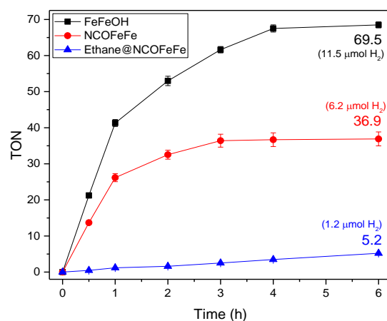
Figure 11. Photocatalytic hydrogen production under standard conditions (0.084 mM of the homogeneous catalyst, 0.5 mM of [\text{Ru}(\text{bpy})_3]^{2+} , 100 mM of ascorbic acid, and 1 M of the acetate buffer
