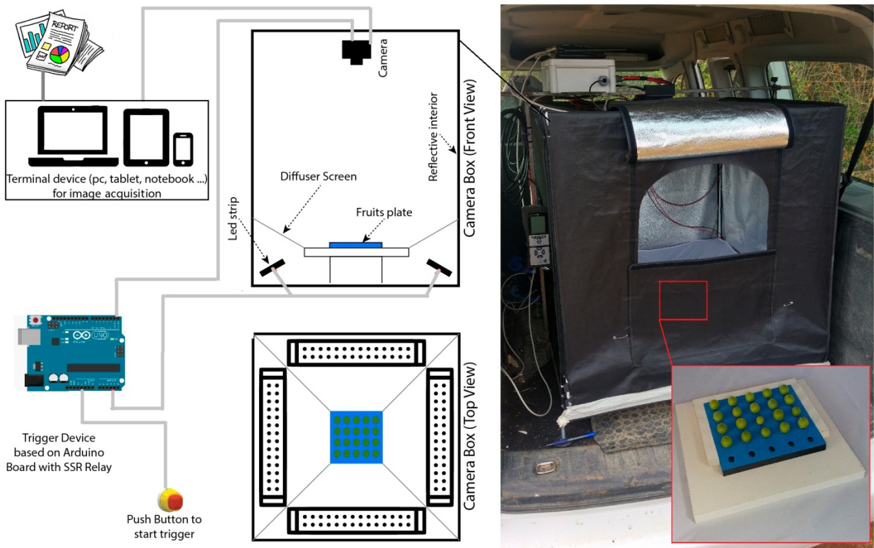
Figure 1. Device (SAEQQ) developed for automatic image acquisition and analysis
