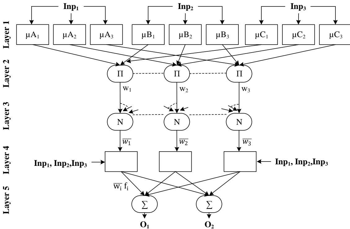
Figure 3. CANFIS structure with three inputs and two outputs.
