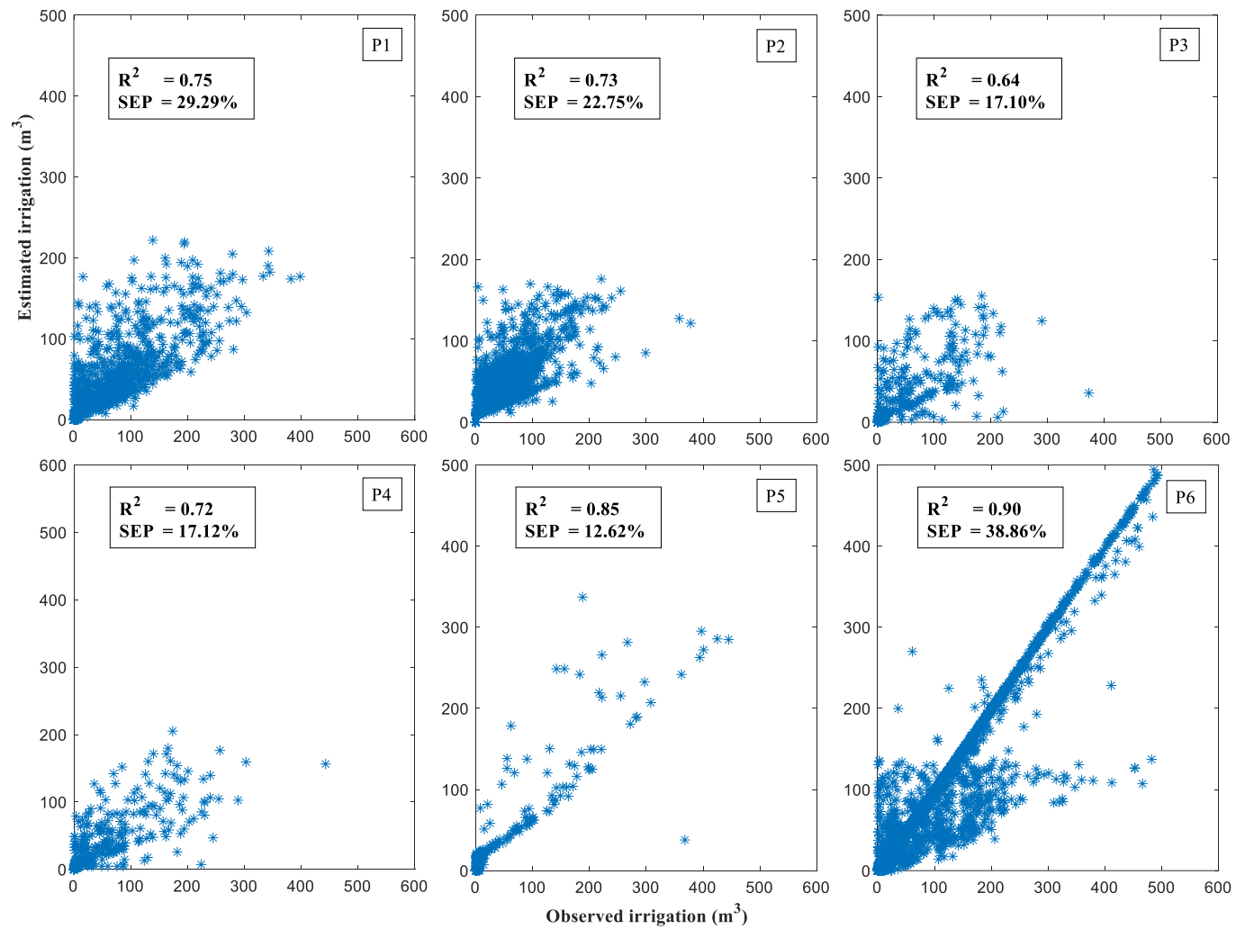
Figure 7. Scatterplots between observed and estimated irrigation volume (test set) applied in each tariff period for I_m model.
