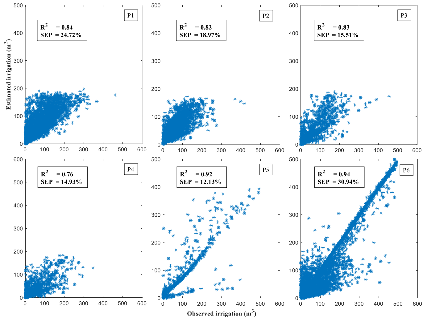
Figure 8. Scatterplots between observed and estimated irrigation volume (test set) applied in each tariff period for I_t model.
