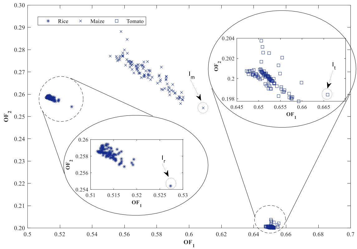
Figure 5. Pareto fronts and best individuals ( I_r , I_m , I_t ) for rice, maize and tomato, respectively.
