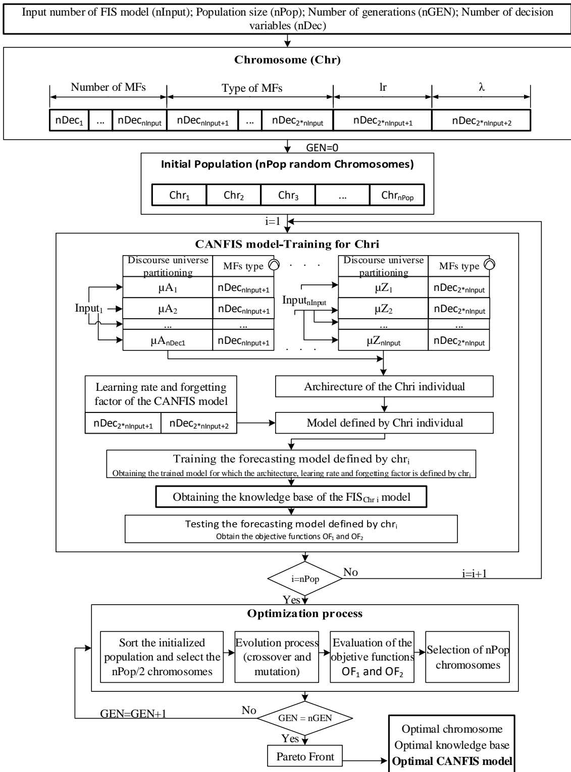
Figure 4. Flowchart of the CANGENFIS model.
