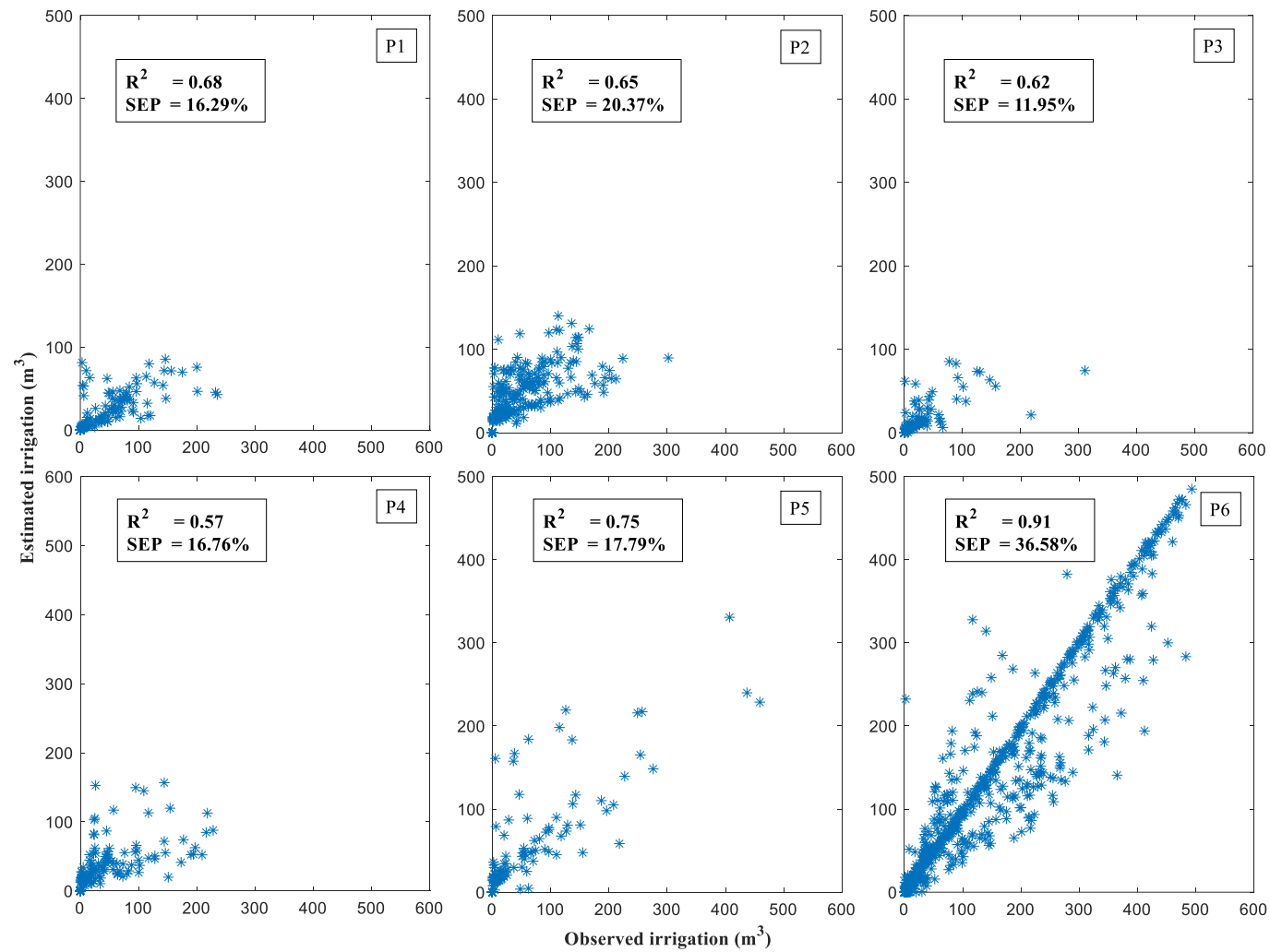
Figure 6. Scatterplots between observed and estimated irrigation volume (test set) applied in each tariff period for I_r model.
