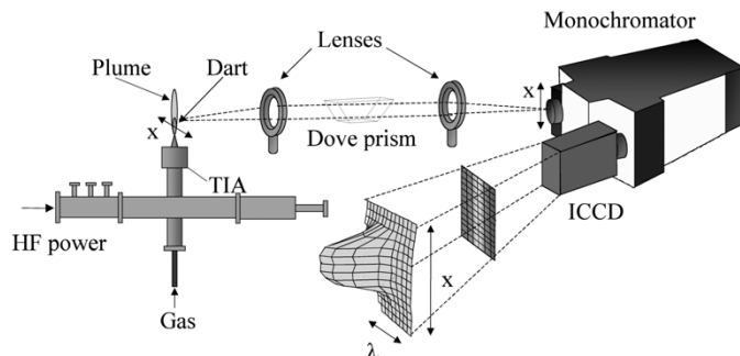
Fig. 1. Experimental setup.
