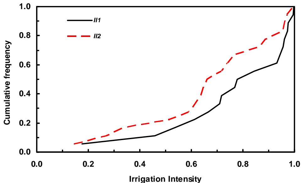
Figure 4.2. Cumulative frequency distributions of irrigation intensity referred to irrigable ( III ) and habilitated ( II2 ) areas.
