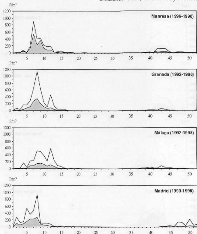
FIGURE 1. Graphical synthesis of the annual dynamics of the Cupressaceae pollen at the REA sites with highest concentrations. For each station and week of the year, the mean concentration and the highest concentration of the period studied are plotted.
