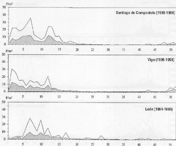
FIGURE 4. Graphical synthesis of the annual dynamics of the Cupressaceae pollen at the REA sites with lower concentrations. For each station and week of the year, the mean concentration and the highest concentration of the period studied are plotted.
