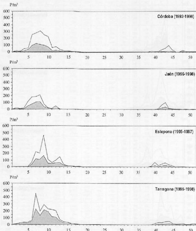
FIGURE 2. Graphical synthesis of the annual dynamics of the Cupressaceae pollen at some of the REA sites with median concentrations. For each station and week of the year, the mean concentration and the highest concentration of the period studied are plotted.
