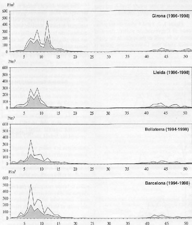
FIGURE 3. Graphical synthesis of the annual dynamics of the Cupressaceae pollen at some of the REA sites with median concentrations. For each station and week of the year, the mean concentration and the highest concentration of the period studied are plotted.
