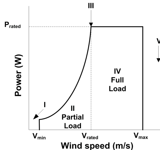
Figure 1. Wind turbine operation modes.
