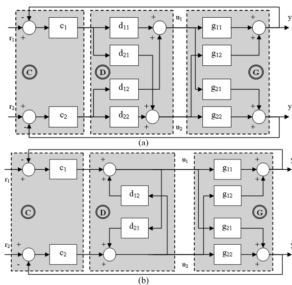
Figure 7. Decoupling control system of a TITO process: (a) conventional decoupling; and (b) inverted decoupling.
