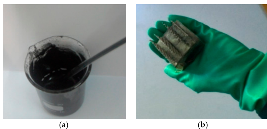
Figure 1. Smart concrete: (a) Dispersion of MWCNT in water for preparation of smart concrete; (b) Cubic sensor made of smart concrete doped with MWCNT.
